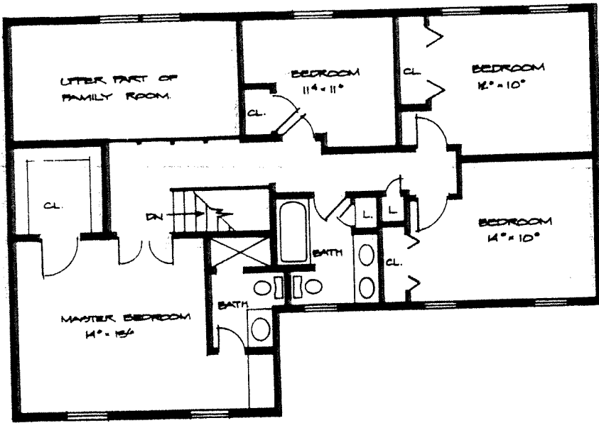
SECOND FLOOR
